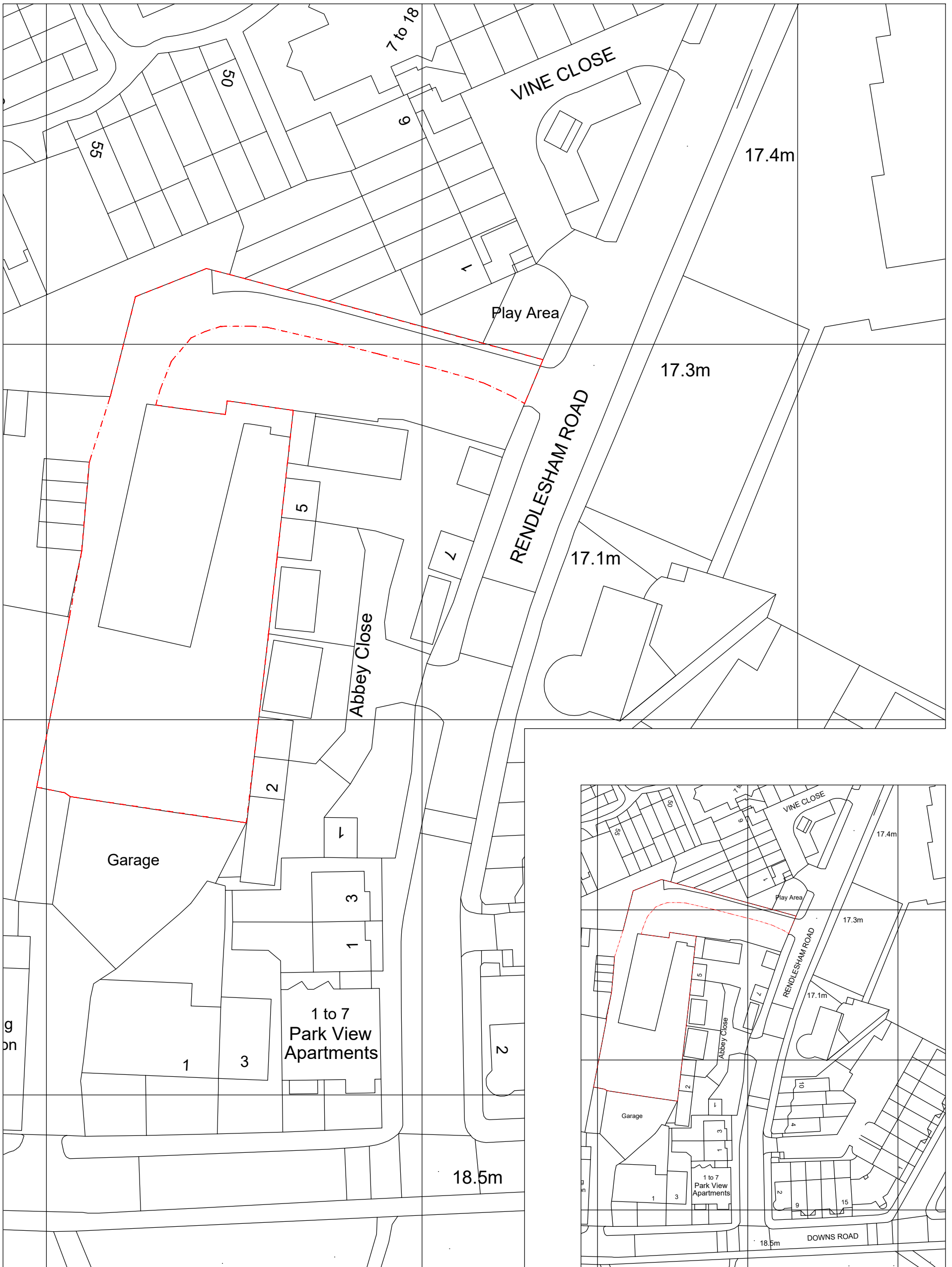
Block Plan - 1:500
